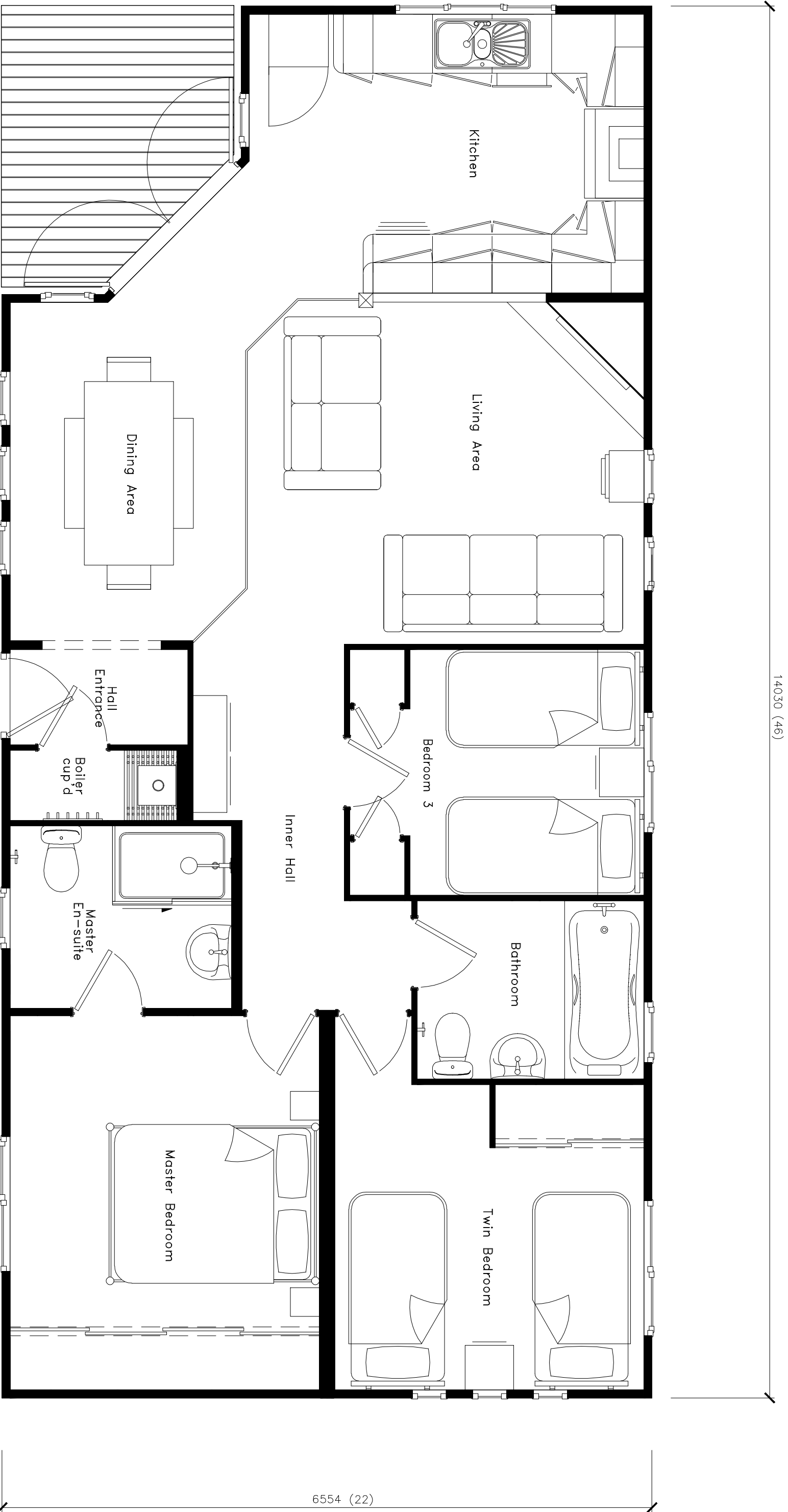
Deckhouse 46x22 Centre Lounge (3 Bed, En-suite)
