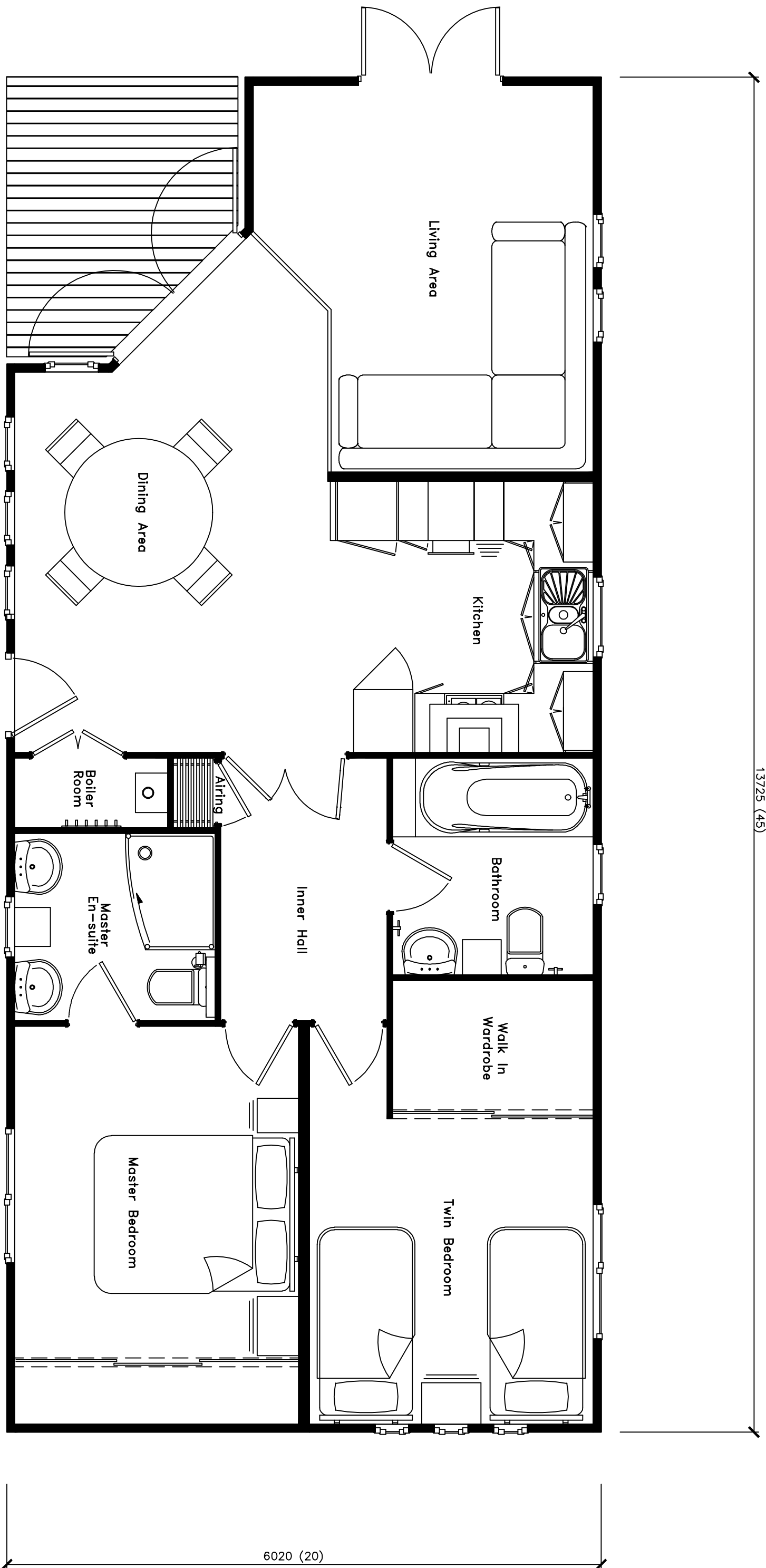
Deckhouse 45x20 Front Lounge (2 Bed, En-suite)
