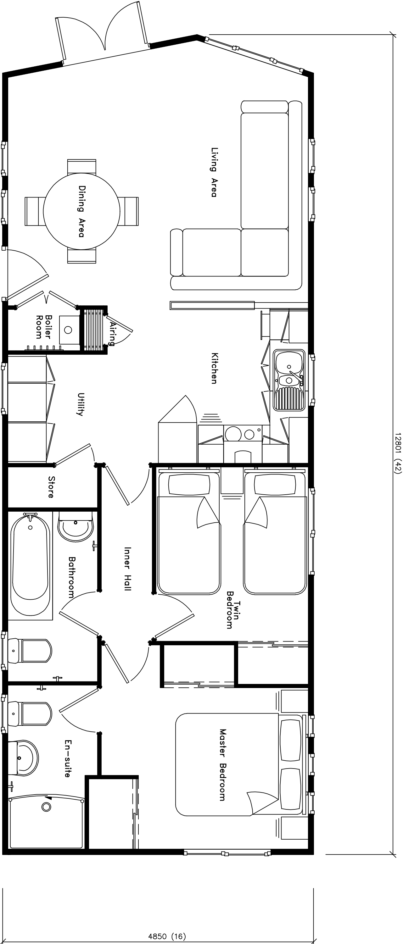
Deckhouse 42x16 (2 Bed, En-suite)
