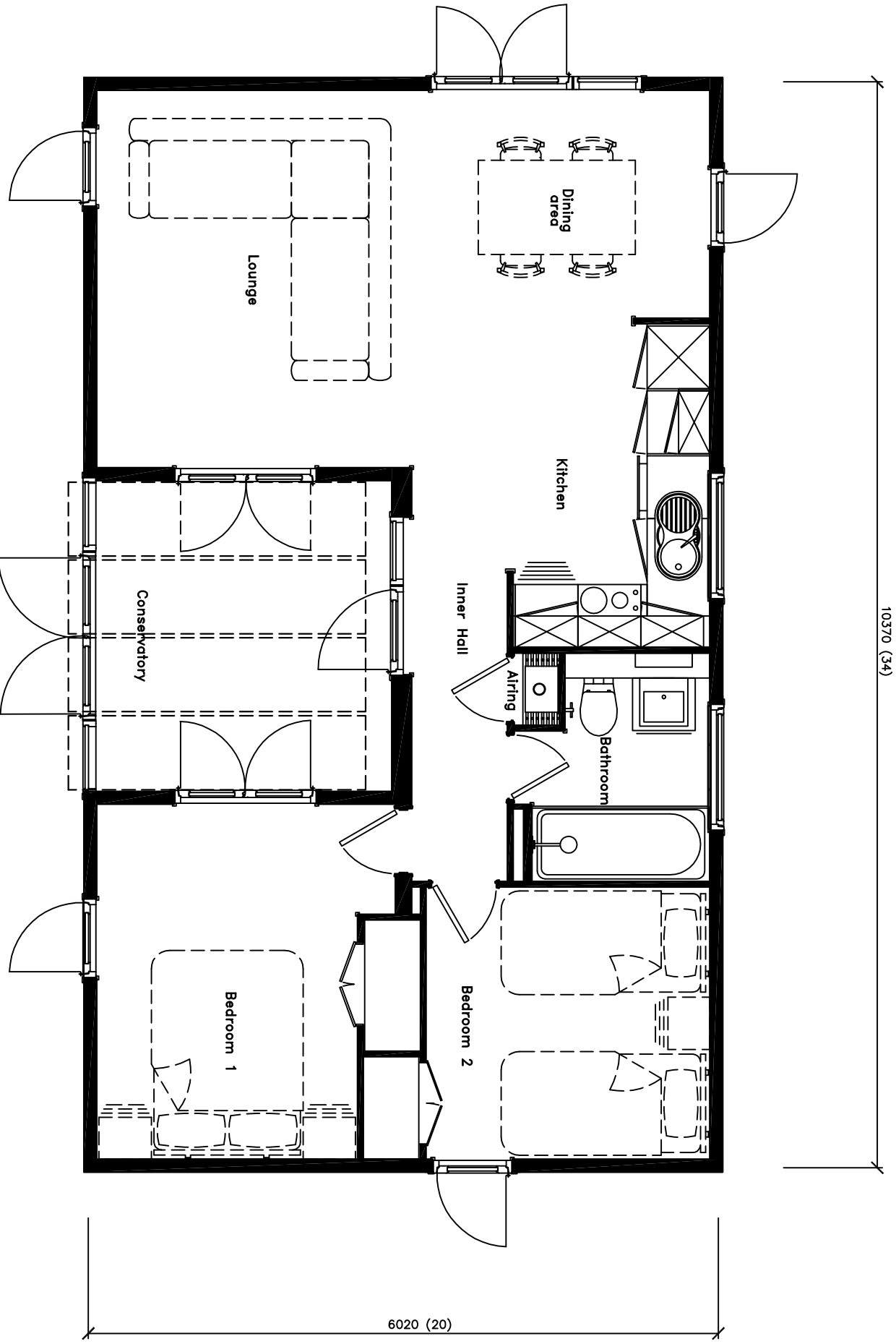
Sanctuary 34x20 (2 Bed, Conservatory) Floor Area 687sq/ft (63.80sq/m)
